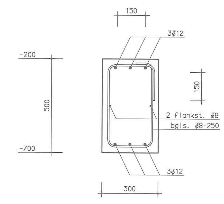
basiswapening balk 300x500
