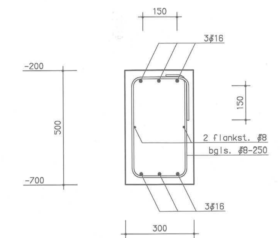
basiswapening balk 300x500
