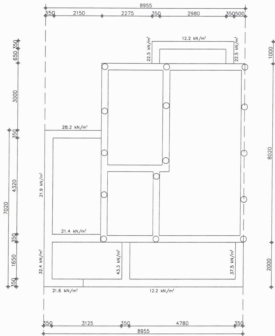
Palenplan – Fundering
