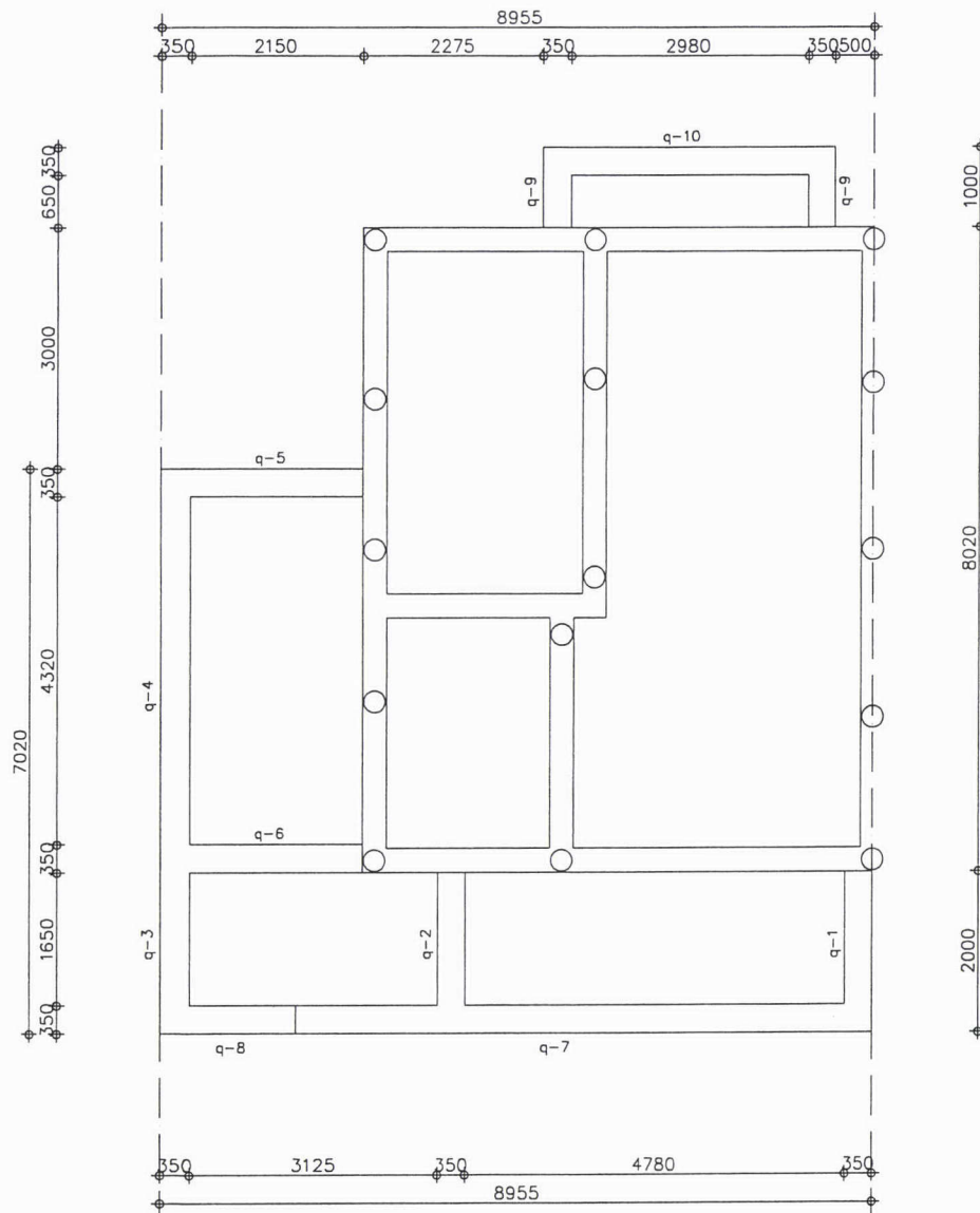
Palenplan - Fundering
